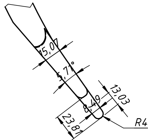
C (1:2)
