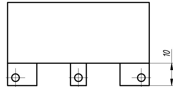
A (1:1)
