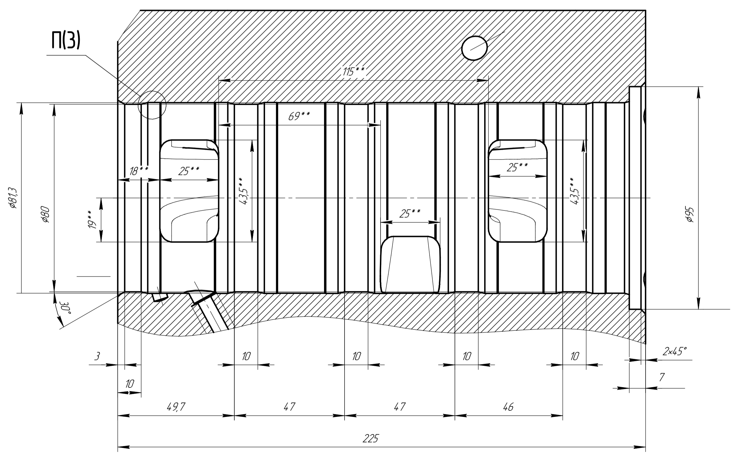
B 1 -B 1 (1:1)(3)
