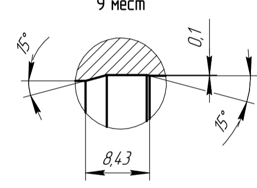
П(2:1)(3)
