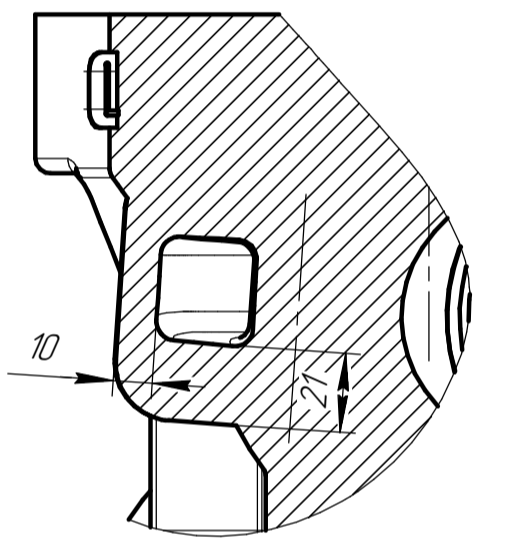
A 2 -A 2 ○(3)
