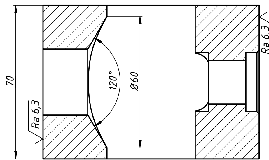
B-B (1:1)
