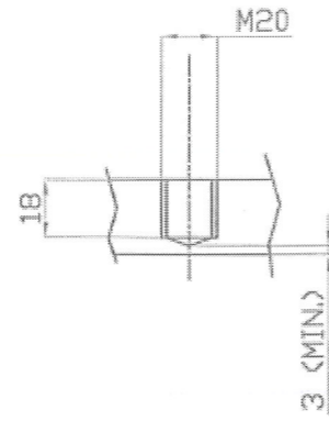
SCREW HOLE FOR EYELIFTING
