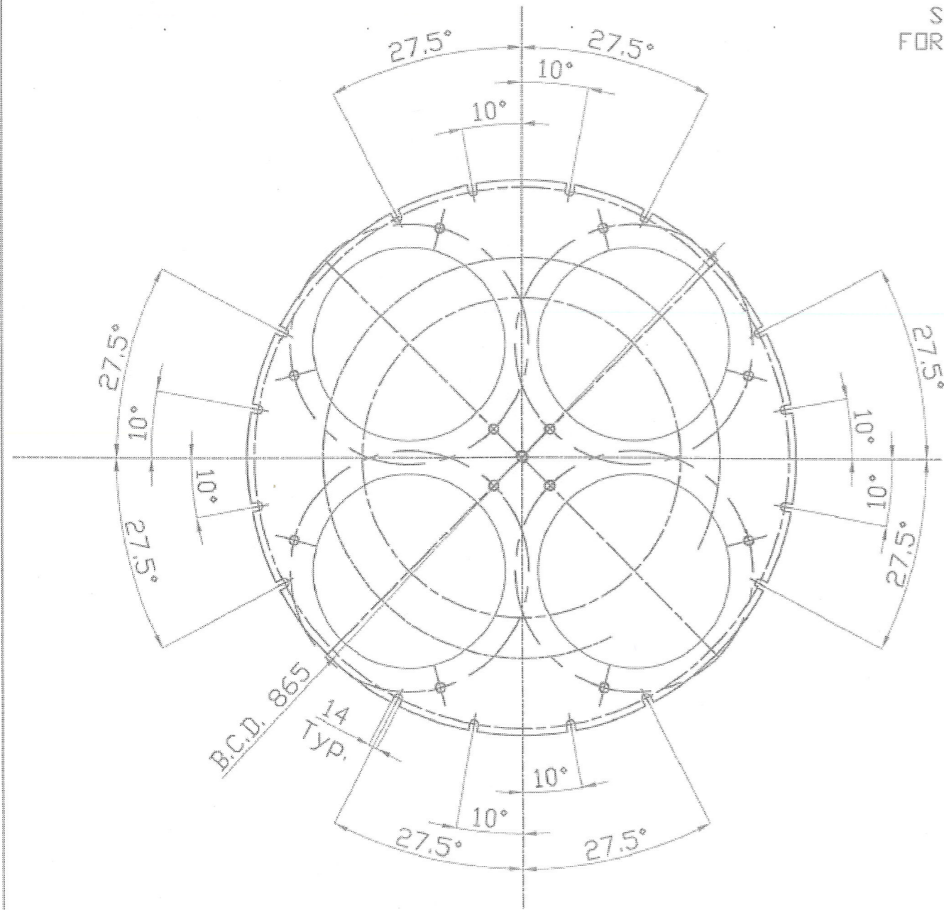
SLOT HOLE POSITION
