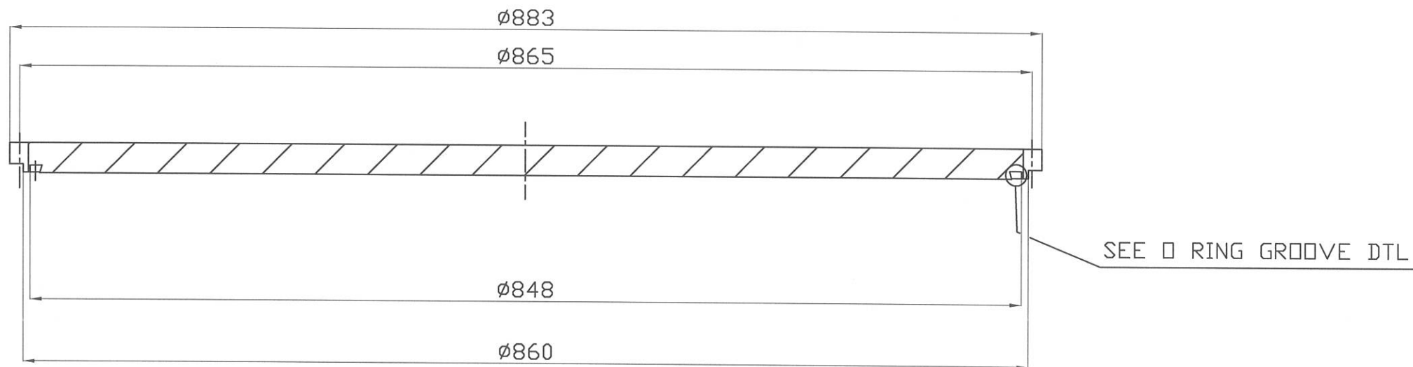
CARTRIDGE SUPPORT PLATE DETAIL
