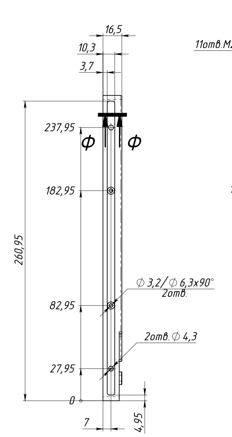
Д (1:1)
